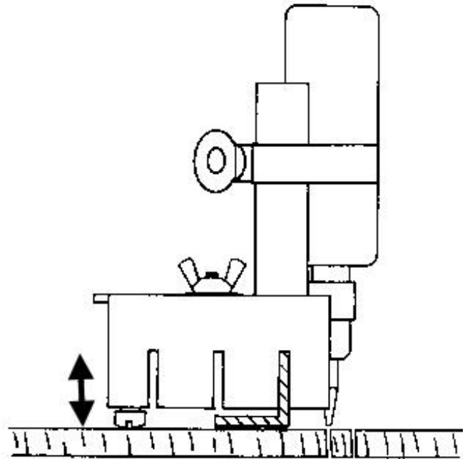
Raise or lower screw feet to adjust tilt for proper alignment of fence and base.
